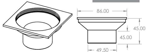
HOUSING D
