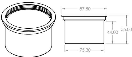
HOUSING E
