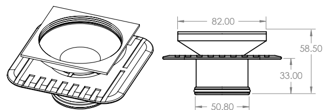
HOUSING H
