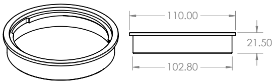
HOUSING A
