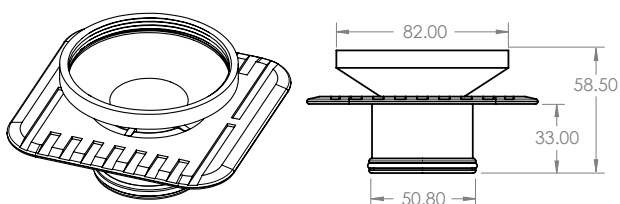
HOUSING G
