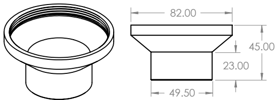
HOUSING C
