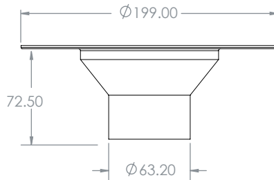
80mm x 50mm Socket
