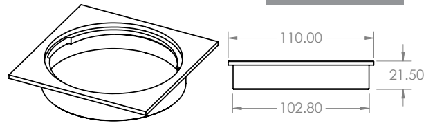
HOUSING B
